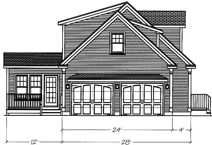
Left Elevation
