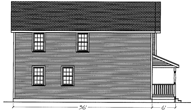
Left Elevation
