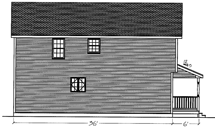
Left Elevation
