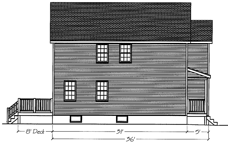
Left Elevation
