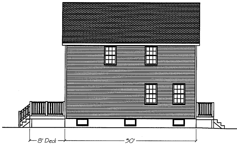
Left Elevation
