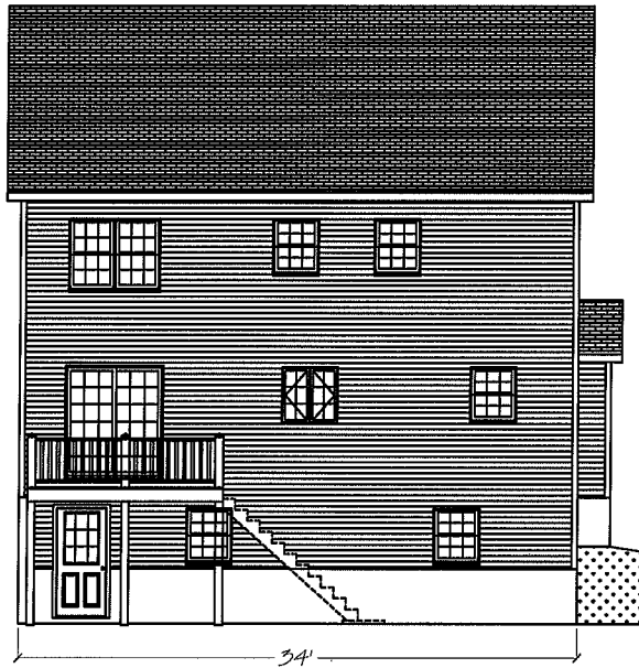
Rear Elevation
