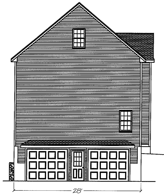
Left Elevation
