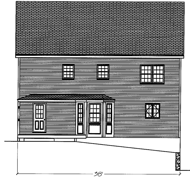
Rear Elevation
