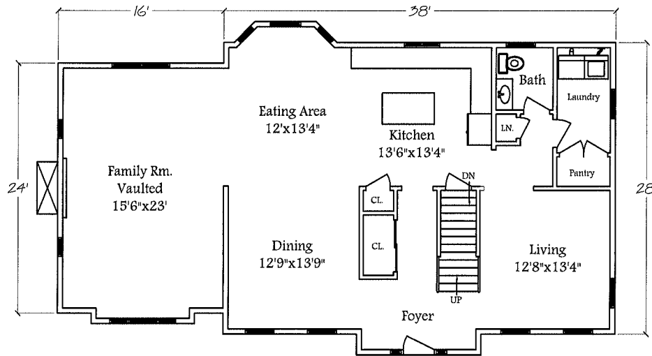
1st Floor Layout
