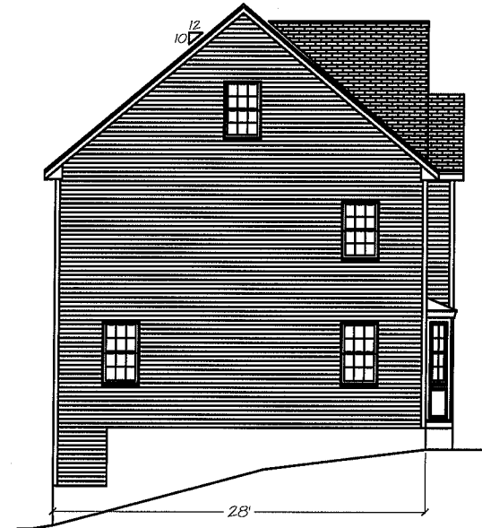
Left Elevation
