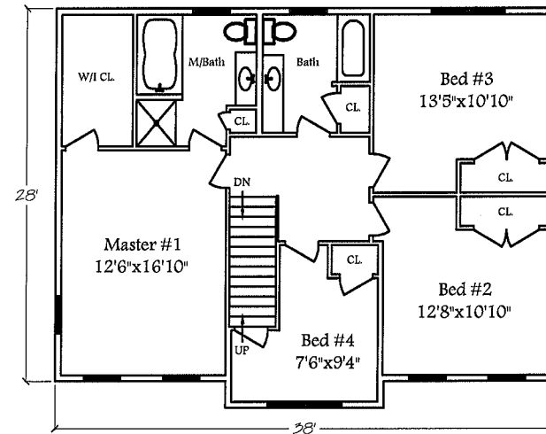
2nd Floor Layout
