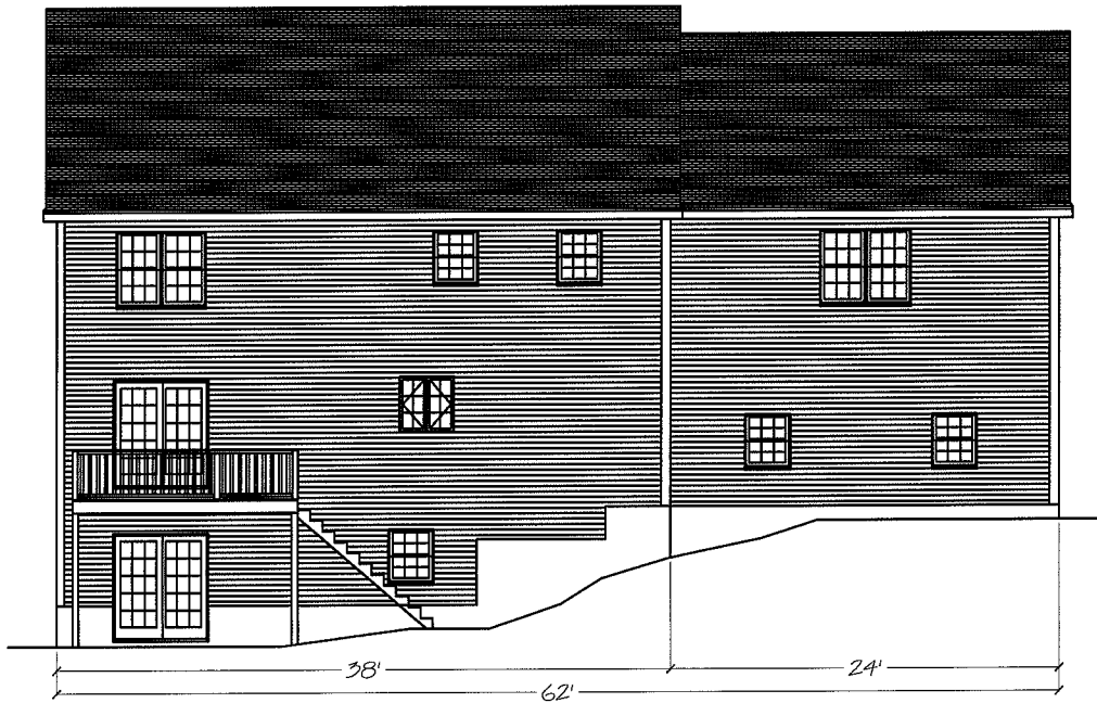
Rear Elevation
