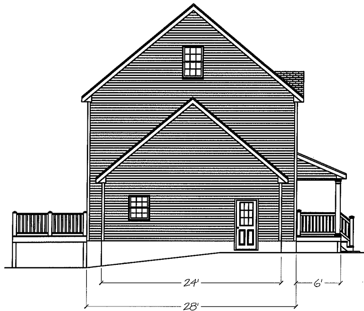
Left Elevation
