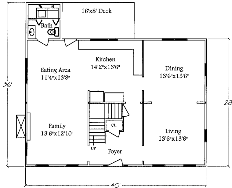
1st Floor Layout
