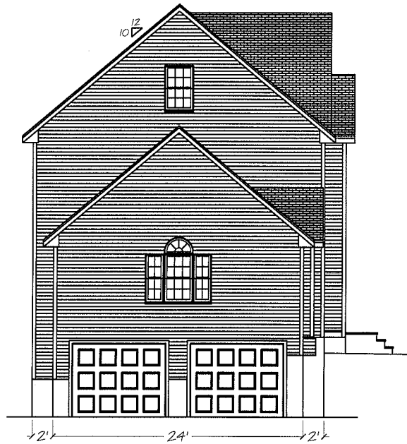
Left Elevation
