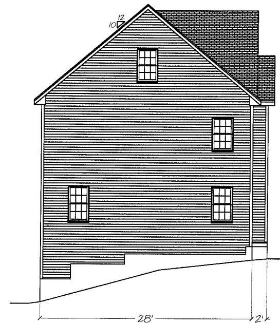
Left Elevation
