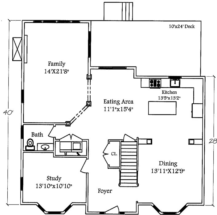
1st Floor Layout
