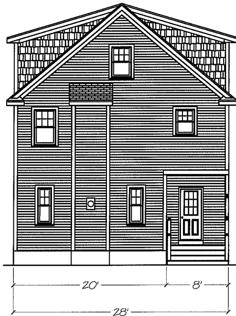
Rear Elevation
