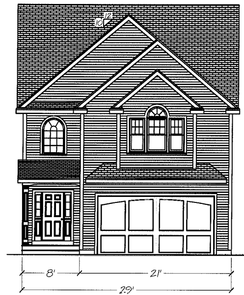
Front Elevation
