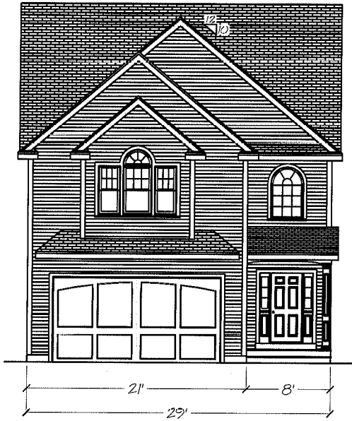
Front Elevation
