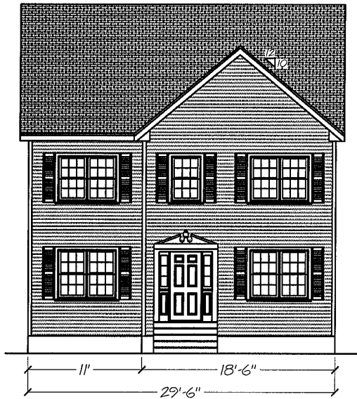
Front Elevation
