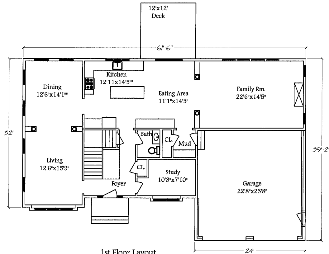
1st Floor Layout
