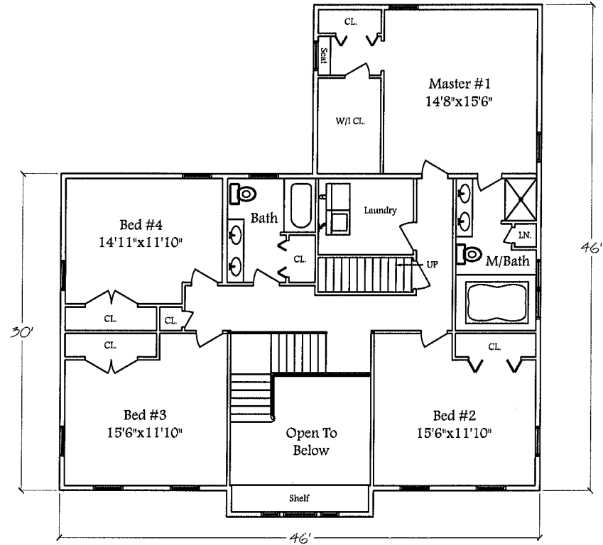
2nd Floor Layout
