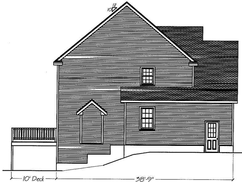
Left Elevation
