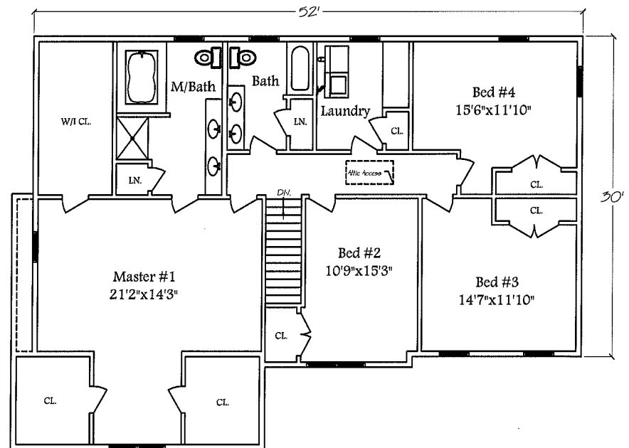
2nd Floor Layout
