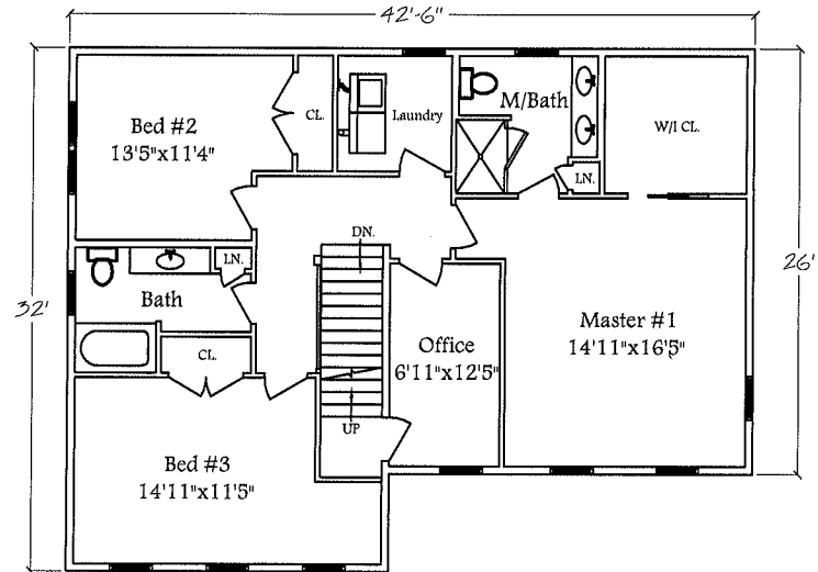
2nd Floor Layout
