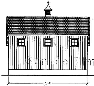
Left Elevation
