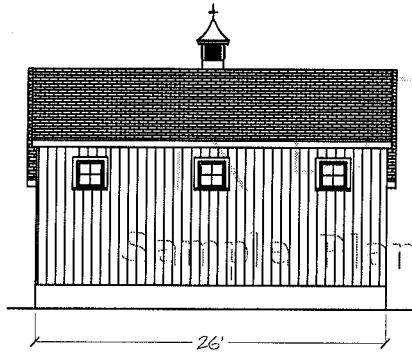
Left Elevation
