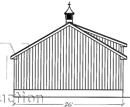
Rear Elevation
