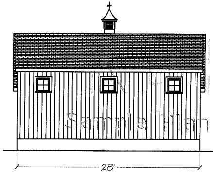
Left Elevation
