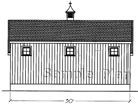
Left Elevation
