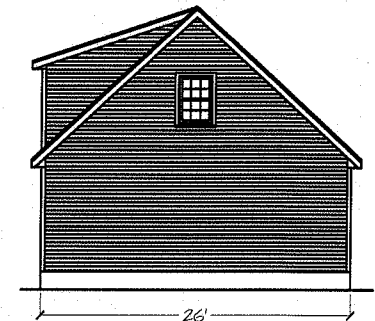
Rear Elevation
