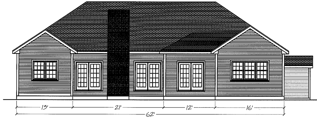
Rear Elevation
