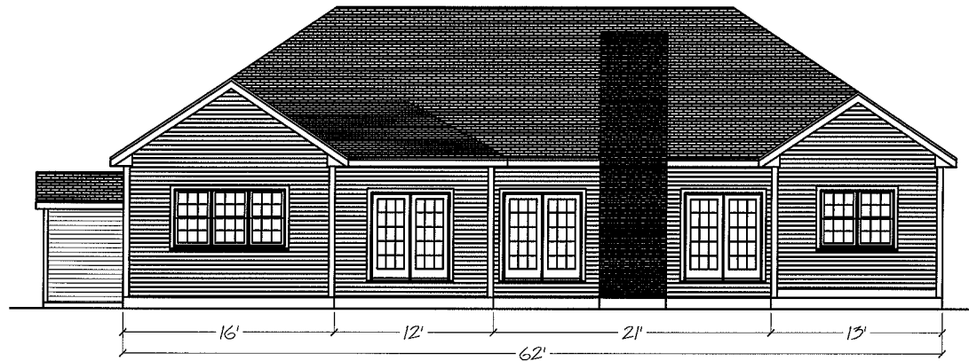
Rear Elevation
