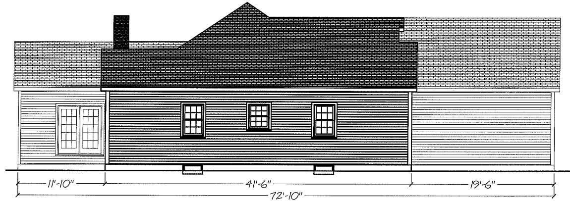
Left Elevation
