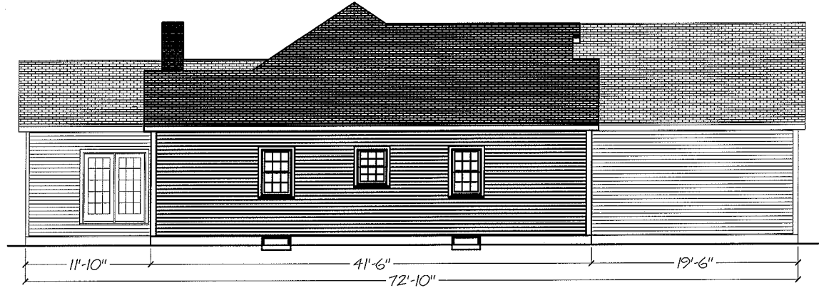
Left Elevation
