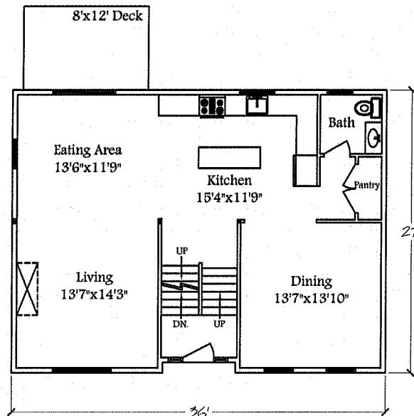
1st Floor Layout
