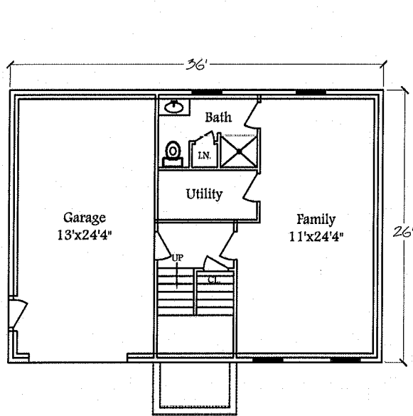
Basement / Garage
