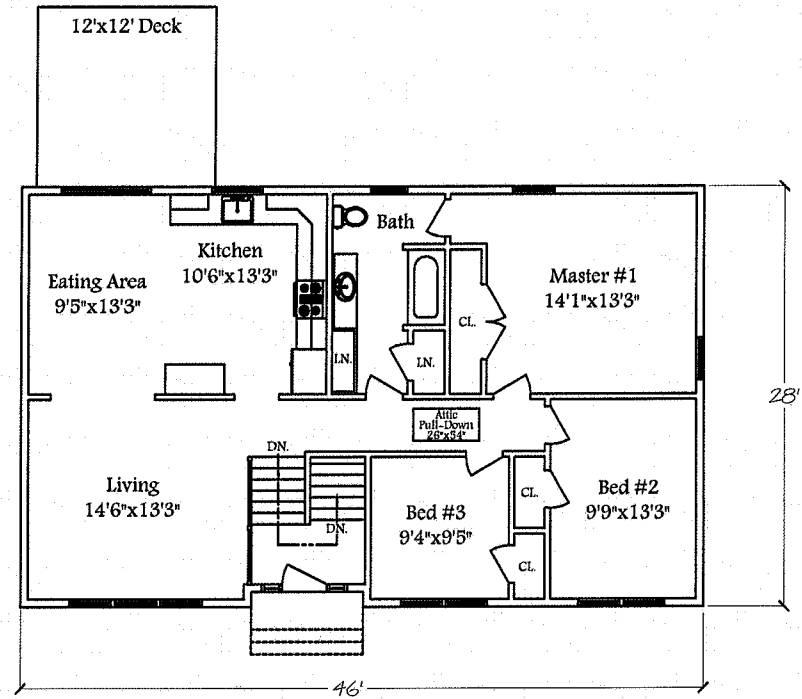
1st Floor Layout
