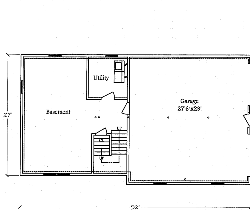
Basement Layout
