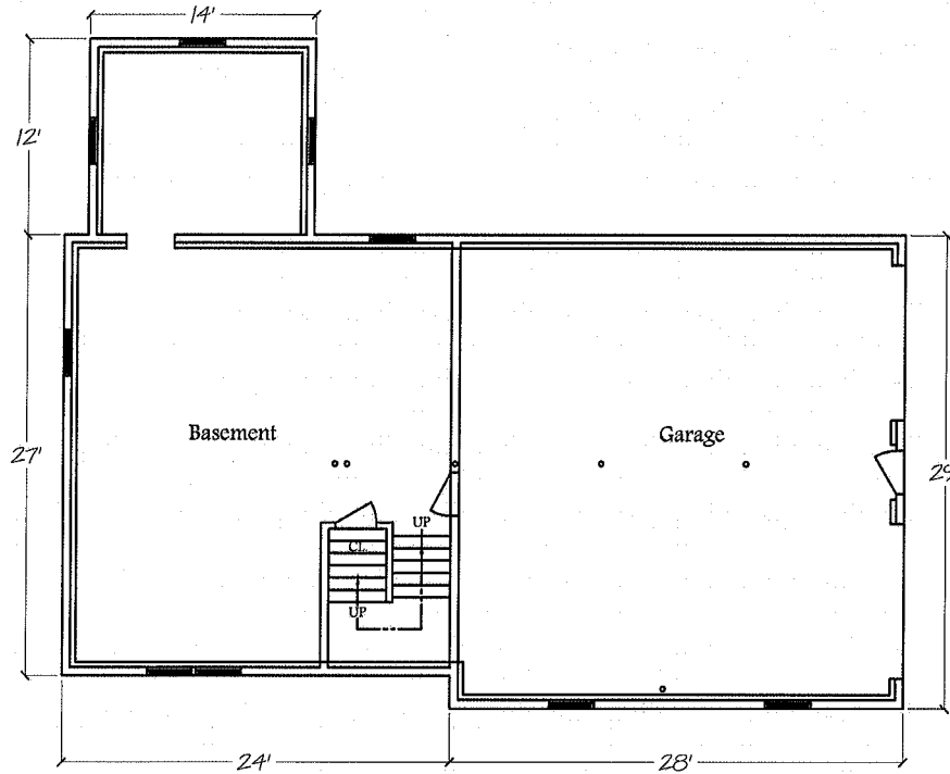
Basement Layout
