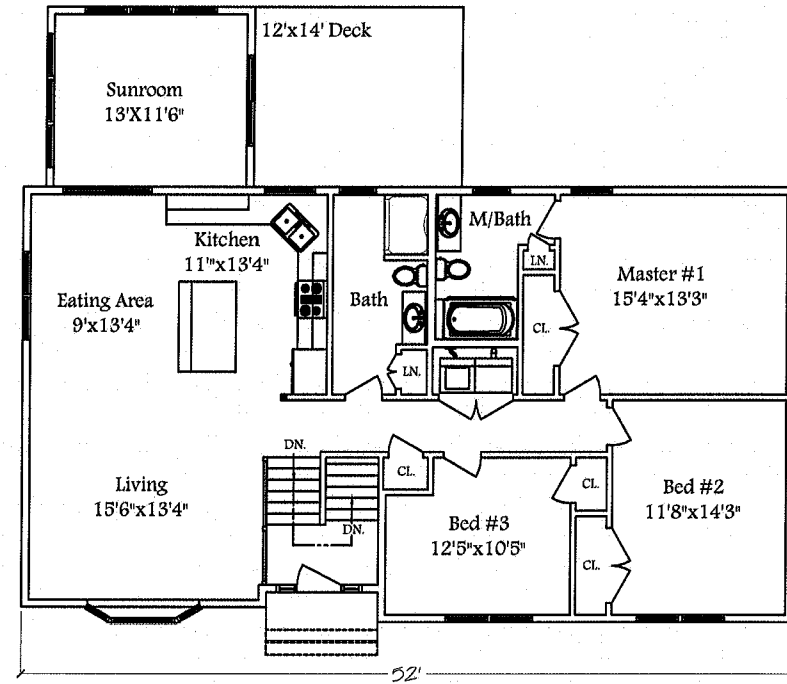
1st Floor Layout
